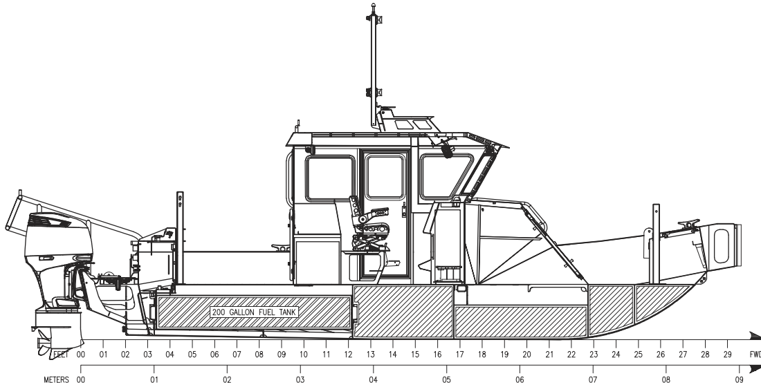
INBOARD PROFILE
