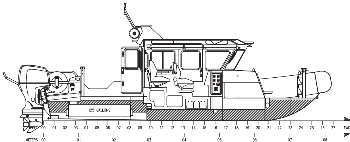
INBOARD PROFILE
