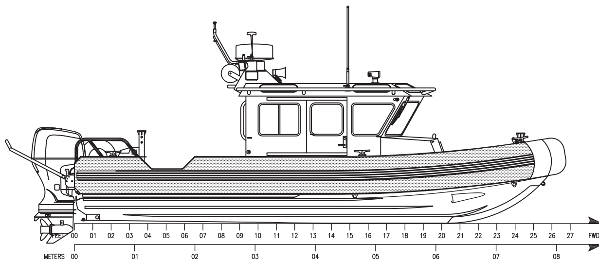
OUTBOARD PROFILE
