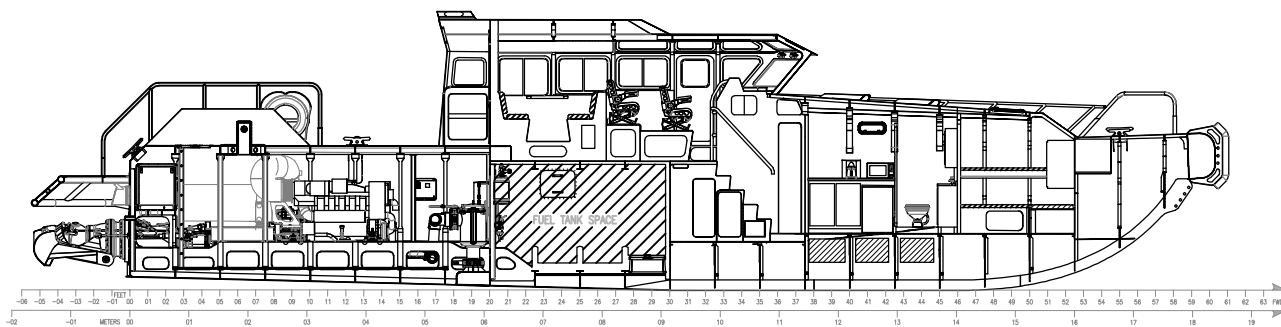
INBOARD PROFILE
