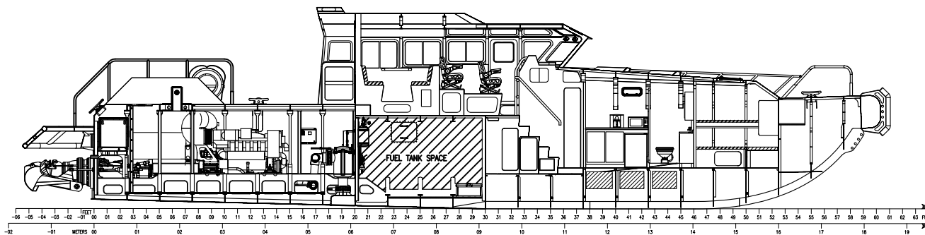
INBOARD PROFILE
