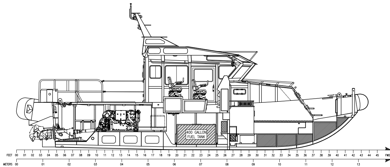
INBOARD PROFILE
