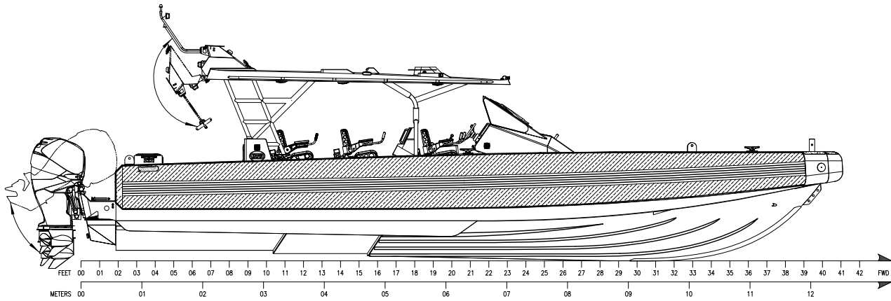
OUTBOARD PROFILE
