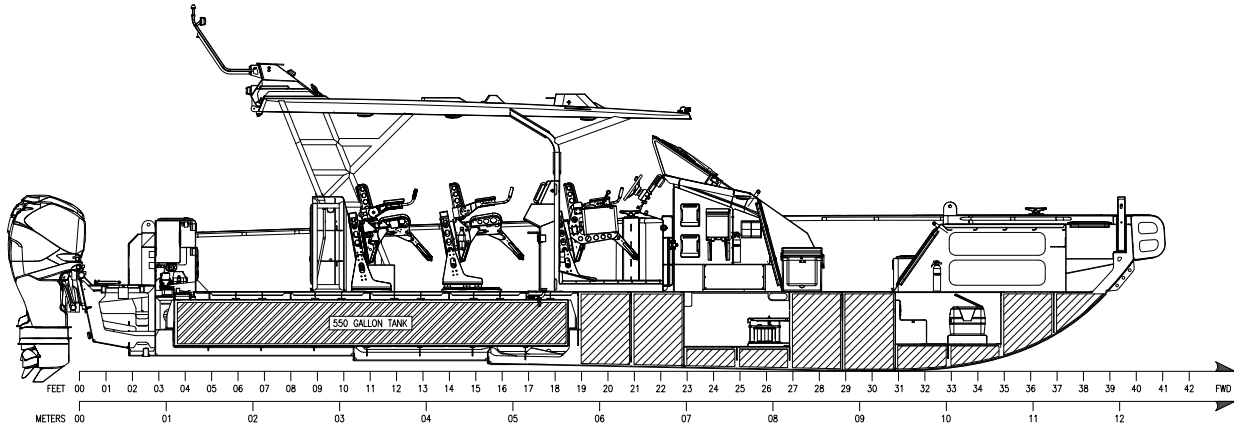
INBOARD PROFILE
