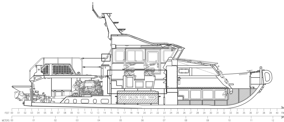
INBOARD PROFILE
