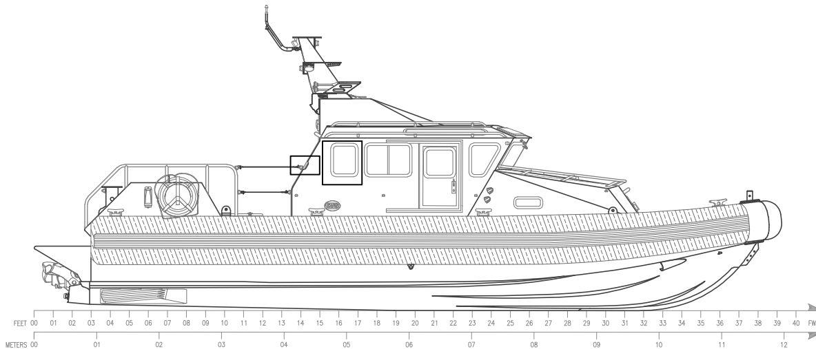
OUTBOARD PROFILE
