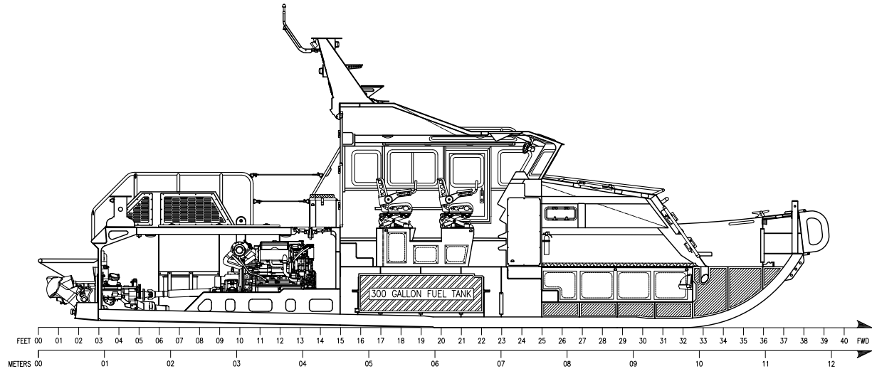
INBOARD PROFILE
