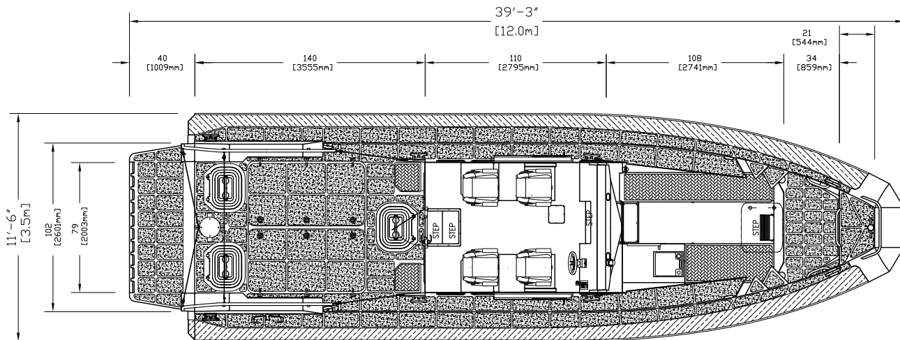
INBOARD PLAN VIEW
