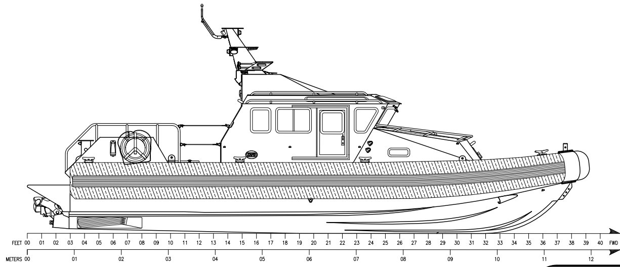
OUTBOARD PROFILE
