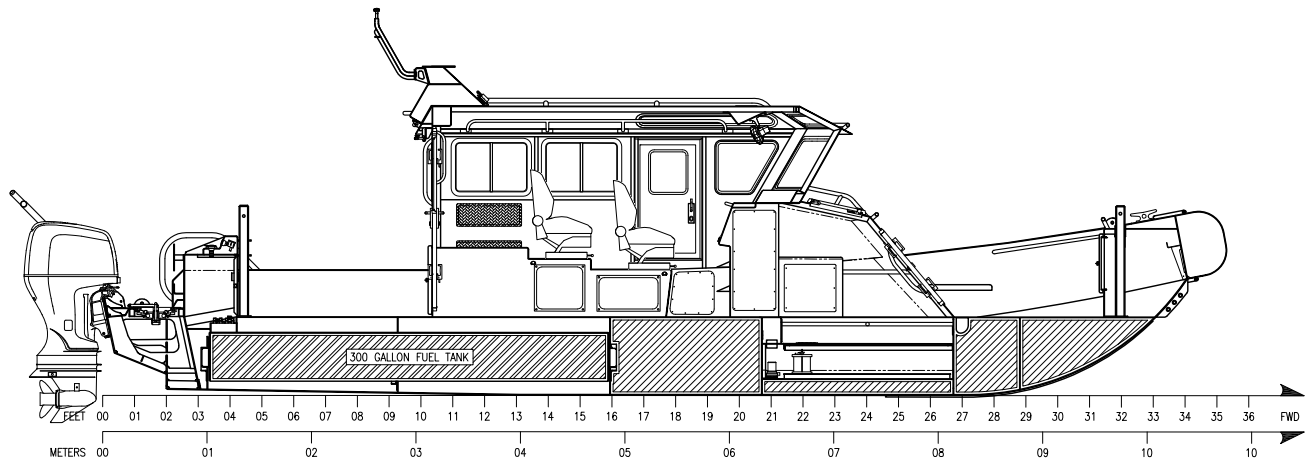
INBOARD PROFILE
