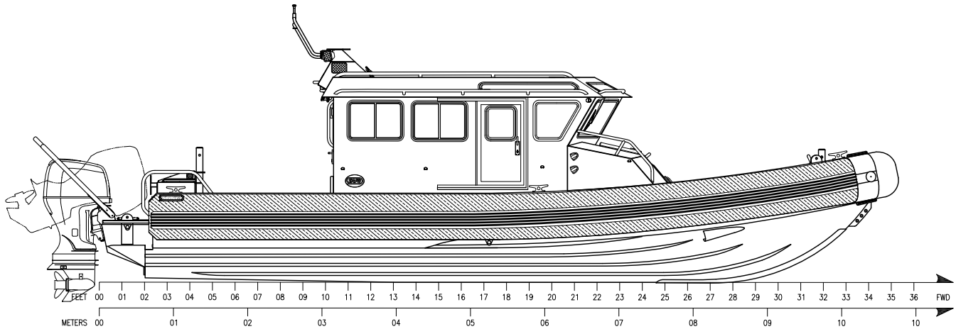
OUTBOARD PROFILE
