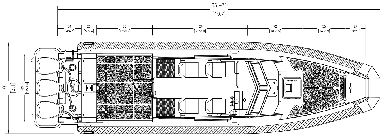
PLAN VIEW
