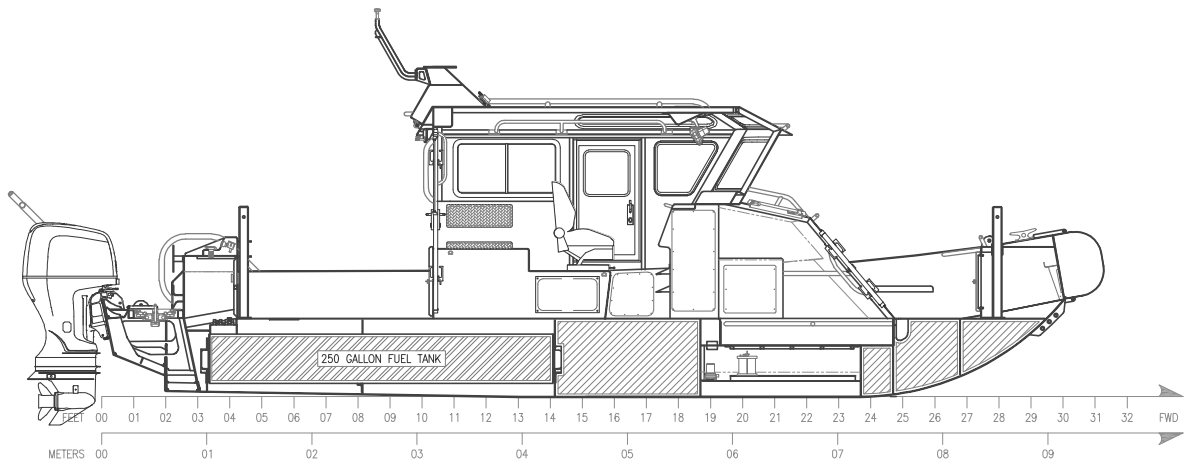
INBOARD PROFILE
