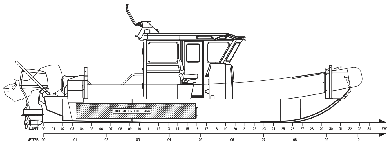
INBOARD PROFILE
