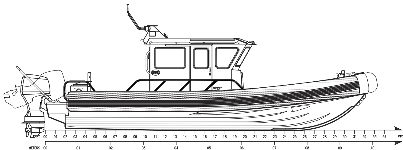
OUTBOARD PROFILE
