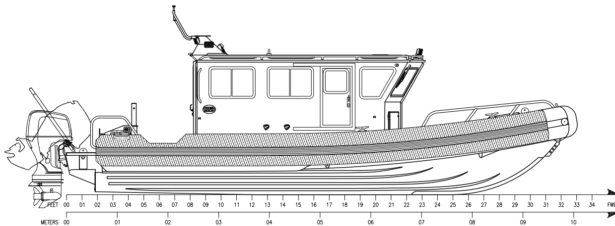
OUTBOARD PROFILE
