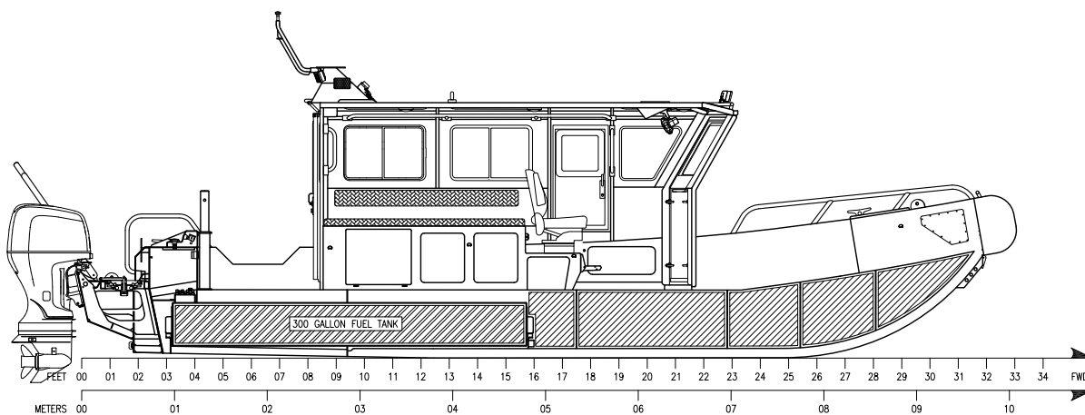
INBOARD PROFILE
