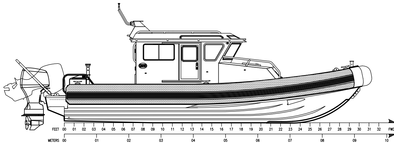
OUTBOARD PROFILE
