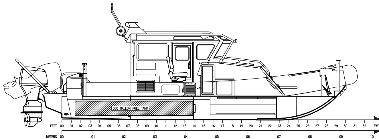
INBOARD PROFILE
