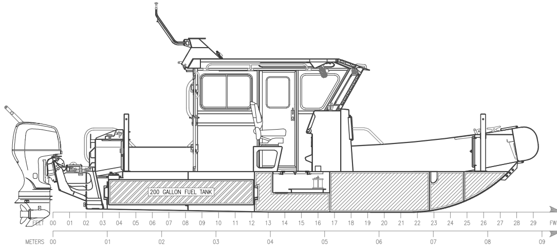
INBOARD PROFILE
