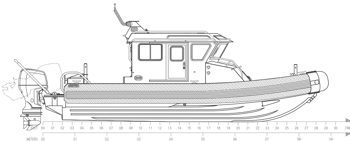
OUTBOARD PROFILE
