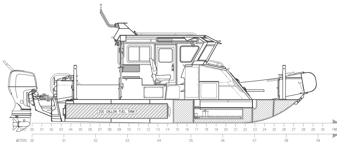
INBOARD PROFILE
