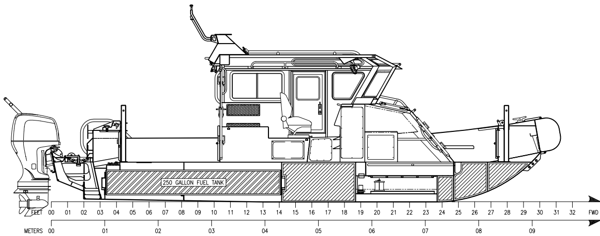
INBOARD PROFILE
