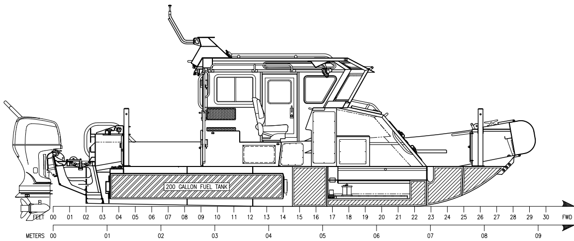
INBOARD PROFILE
