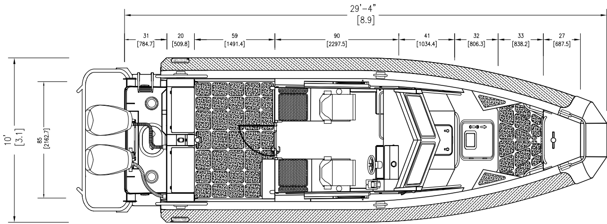
INBOARD PLAN VIEW
