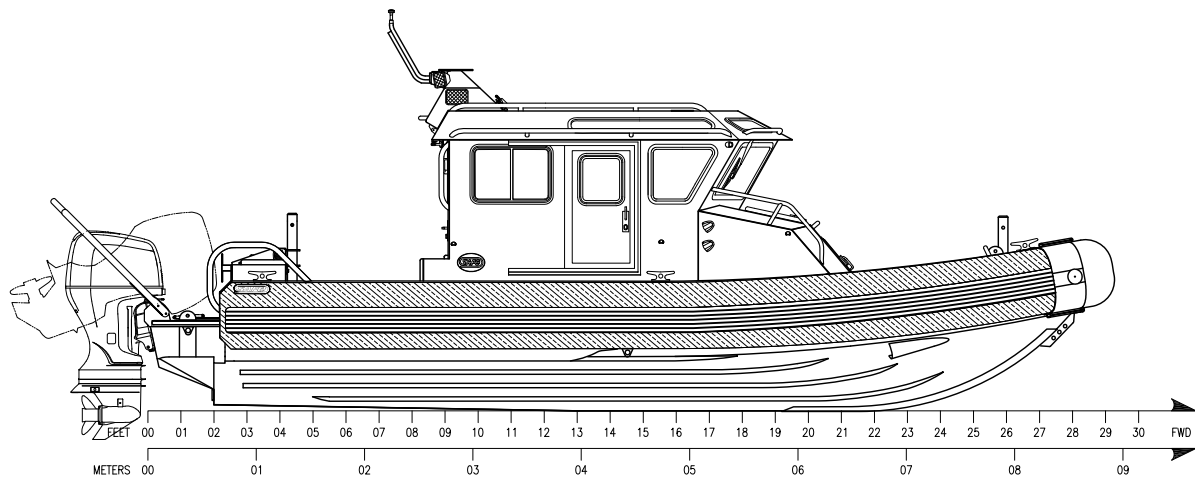
OUTBOARD PROFILE
